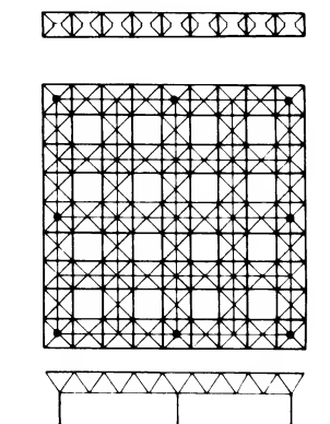
⑭ Space frame structure
